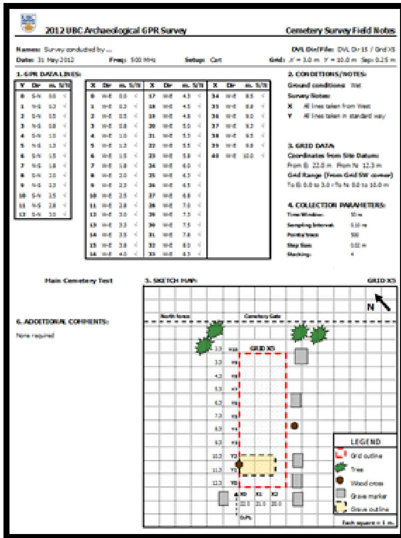
Fig 1. Example GPR Field Notes Log
